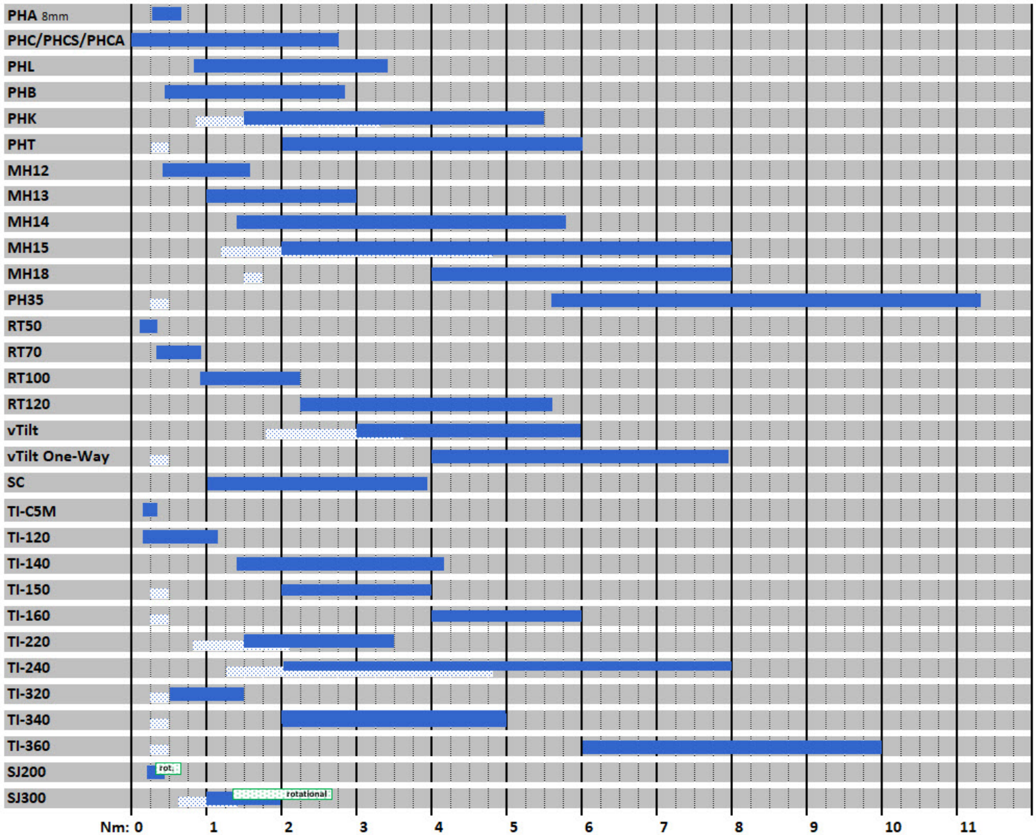
Torque Range Chart
